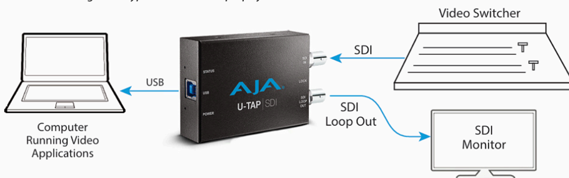
Figure 6. Typical U-TAP SDI Laptop System Connections
