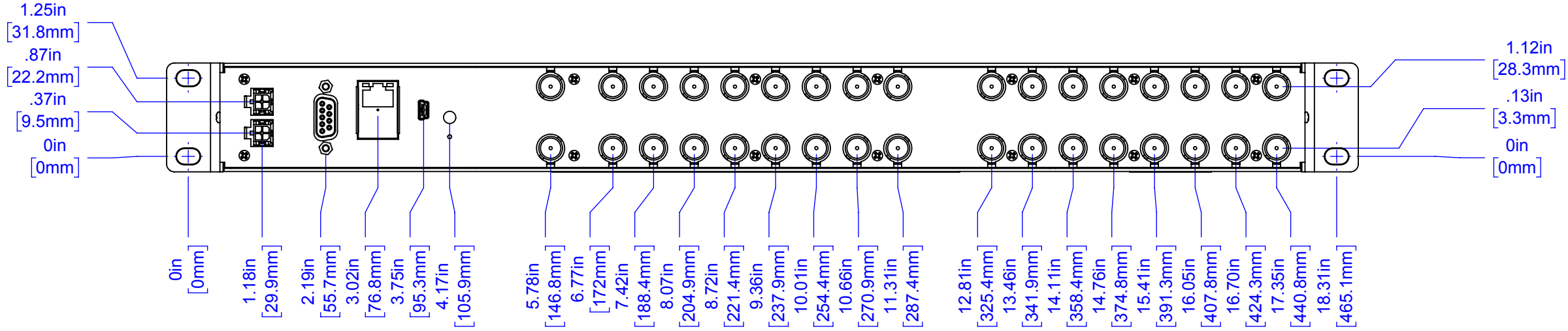
VIEW A-A BACK VIEW
